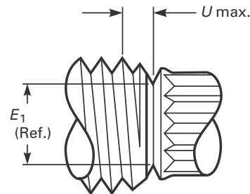
Fig. 1 Groove Diameter
